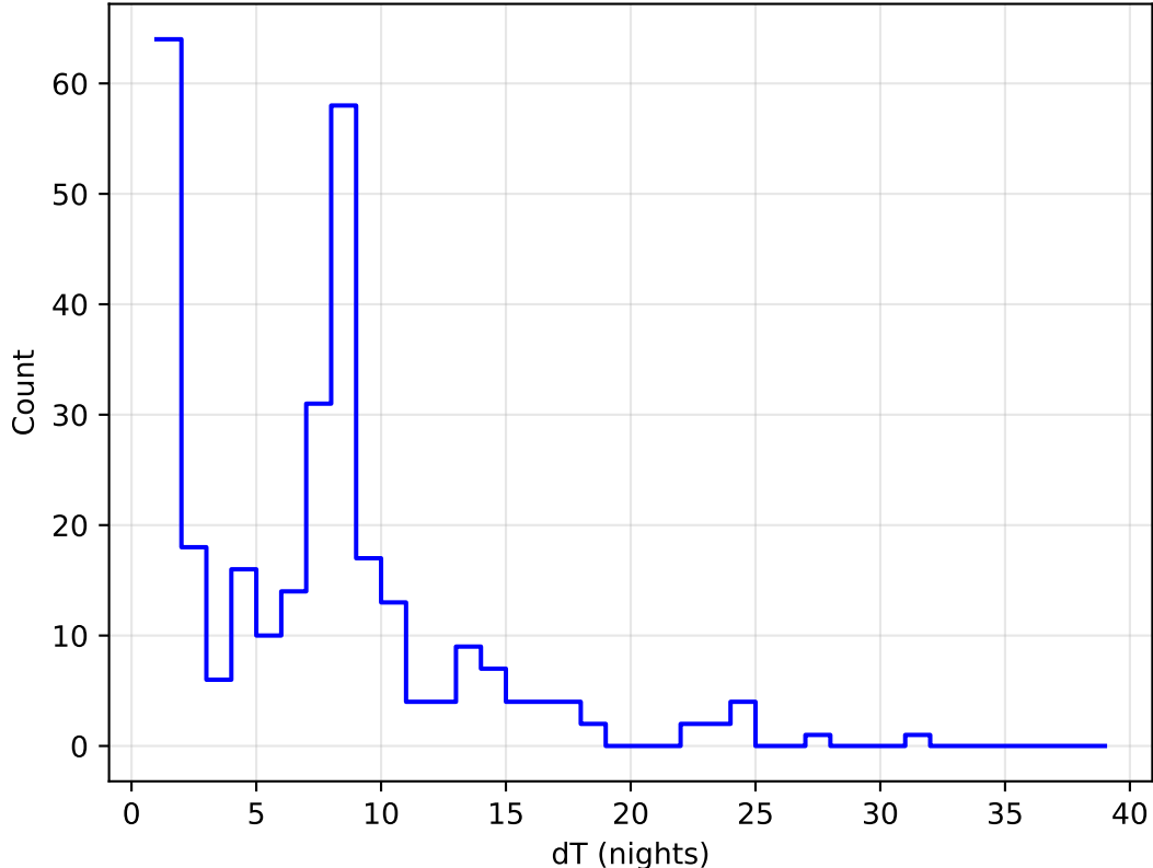
too_elab_heavy_r128_d3_ugrizy_v3.4_10yrs all bands: DD:XMM_LSS Delta Nights Histogram
