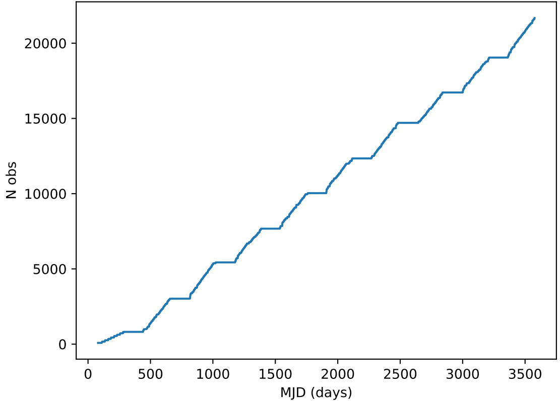
too_elab_heavy_r128_d3_ugrizy_v3.4_10yrs all bands: DD:XMM_LSS Cumulative NVisits
