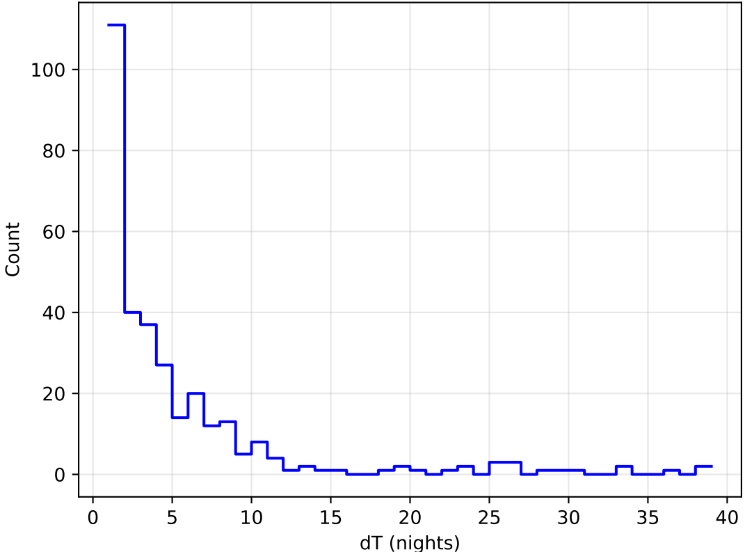
too_elab_heavy_r128_d3_ugrizy_v3.4_10yrs all bands: DD:WFD Delta Nights Histogram
