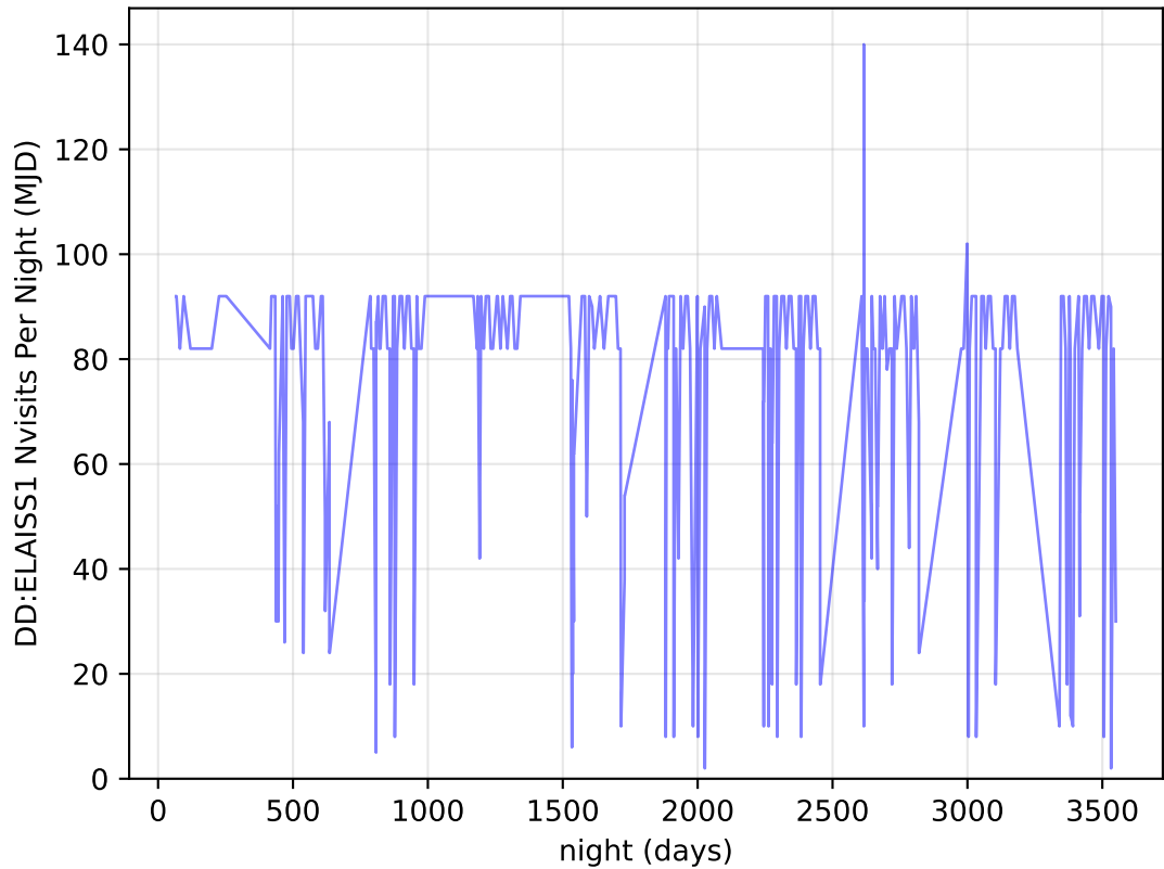
too_elab_heavy_r128_d3_ugrizy_v3.4_10yrs all bands: DD:ELAISS1 Nvisits Per Night
