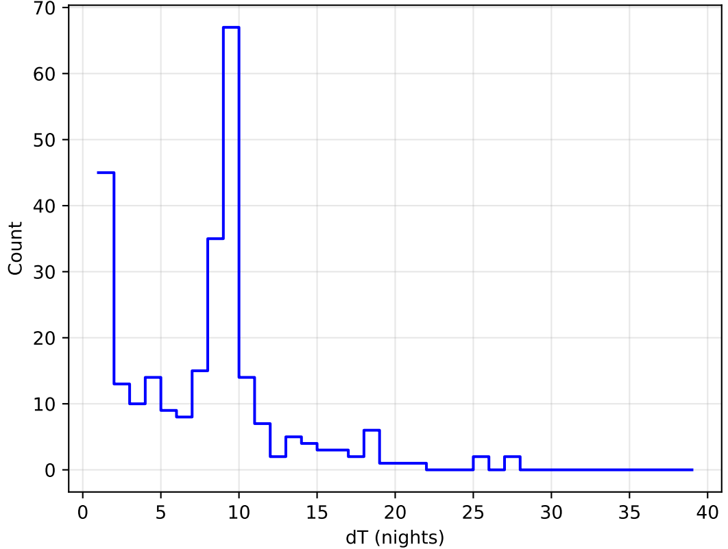
too_elab_heavy_r128_d3_ugrizy_v3.4_10yrs all bands: DD:ELAISS1 Delta Nights Histogram
