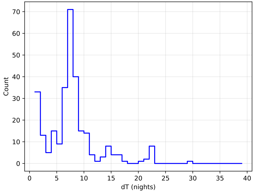
too_elab_heavy_r128_d3_ugrizy_v3.4_10yrs all bands: DD:EDFS Delta Nights Histogram
