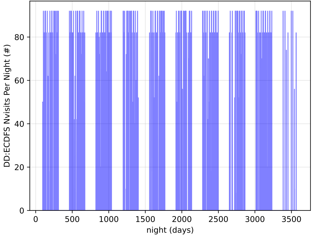
too_elab_heavy_r128_d3_ugrizy_v3.4_10yrs all bands: DD:ECDFS Nvisits Per Night
