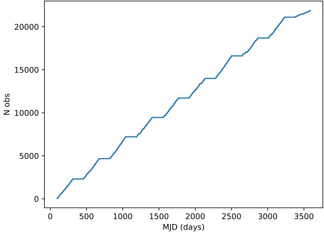
too_elab_heavy_r128_d3_ugrizy_v3.4_10yrs all bands: DD:ECDFS Cumulative NVisits
