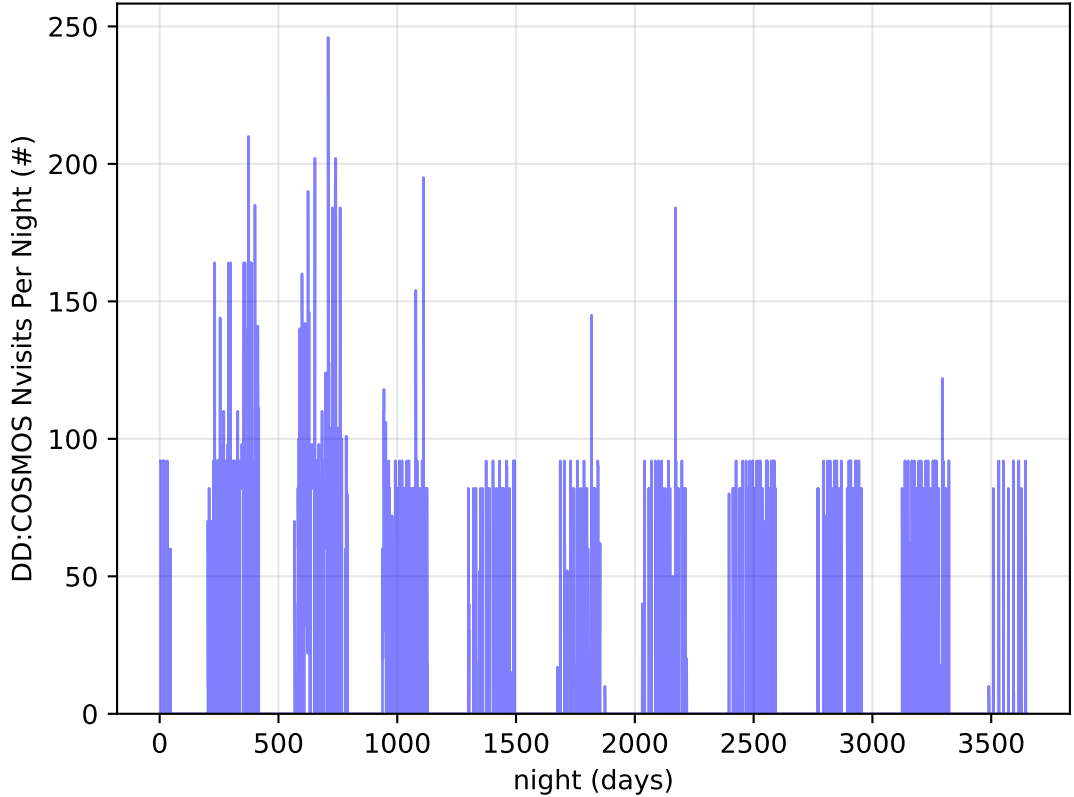
too_elab_heavy_r128_d3_ugrizy_v3.4_10yrs all bands: DD:COSMOS Nvisits Per Night
