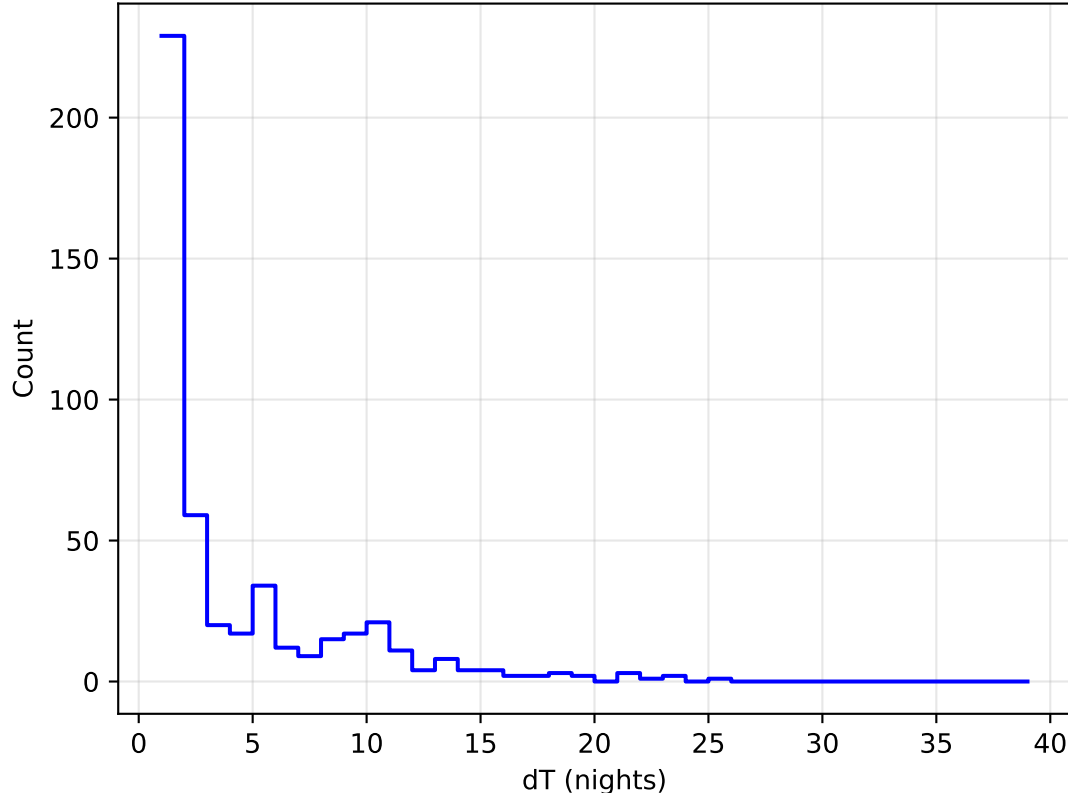
too_elab_heavy_r128_d3_ugrizy_v3.4_10yrs all bands: DD: COSMOS Delta Nights Histogram
