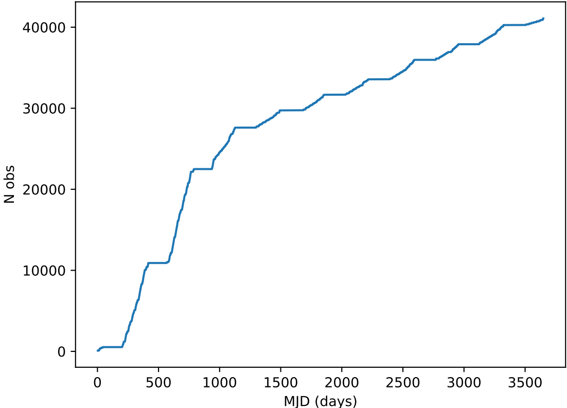
too_elab_heavy_r128_d3_ugrizy_v3.4_10yrs all bands: DD: COSMOS Cumulative NVisits
