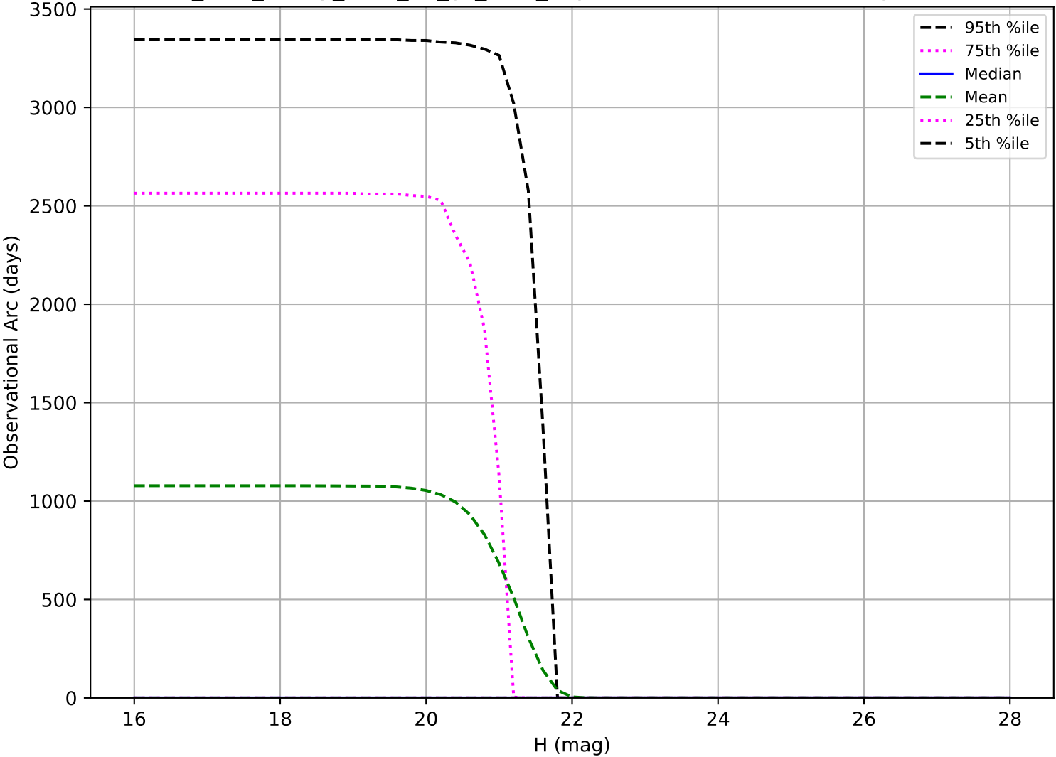
too_elab_heavy_r128_d3_gz_v3.4_10yrs: Observational Arc Length Vatira
