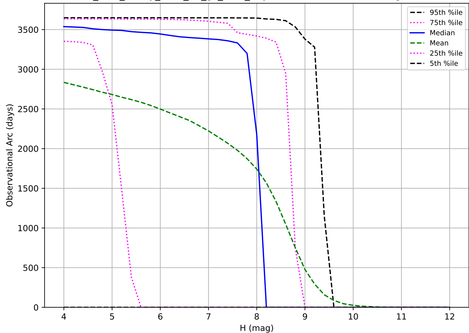
too_elab_heavy_r128_d3_gz_v3.4_10yrs: Observational Arc Length TNO
