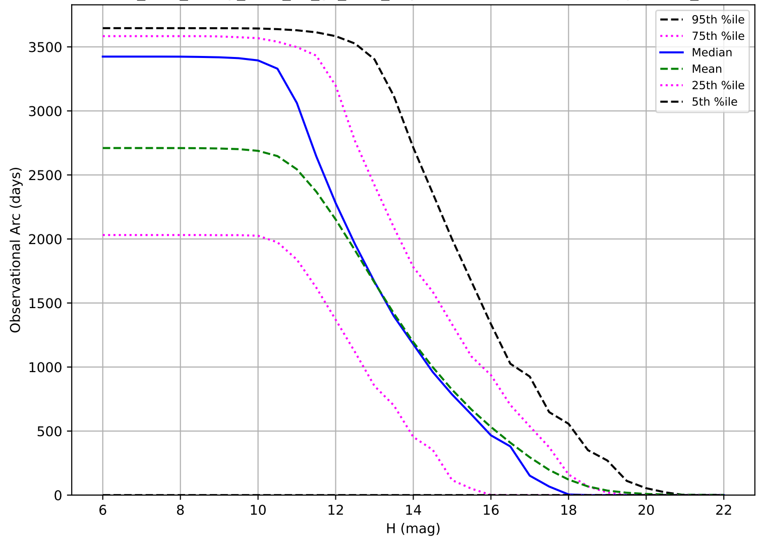
too_elab_heavy_r128_d3_gz_v3.4_10yrs: Observational Arc Length OCC_r5
