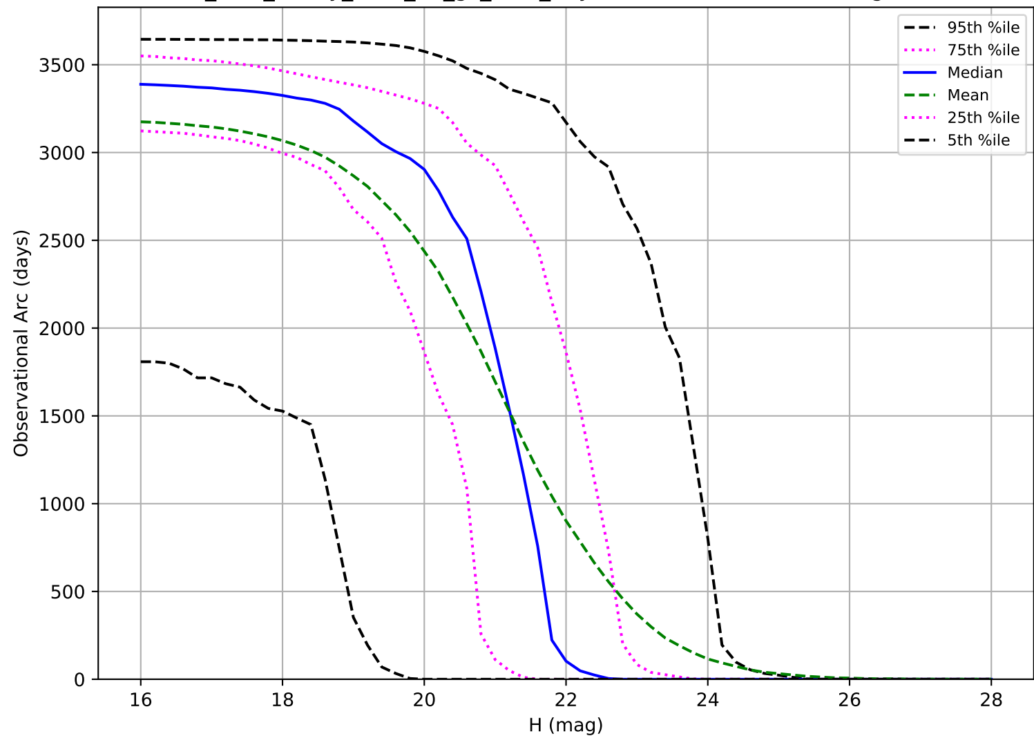
too_elab_heavy_r128_d3_gz_v3.4_10yrs: Observational Arc Length NEO
