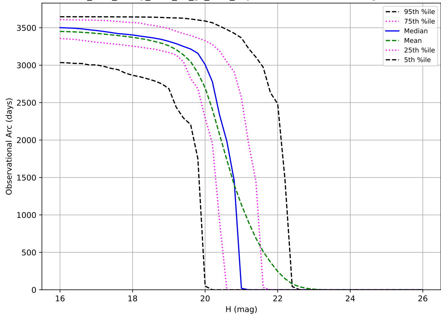
too_elab_heavy_r128_d3_gz_v3.4_10yrs: Observational Arc Length MBA
