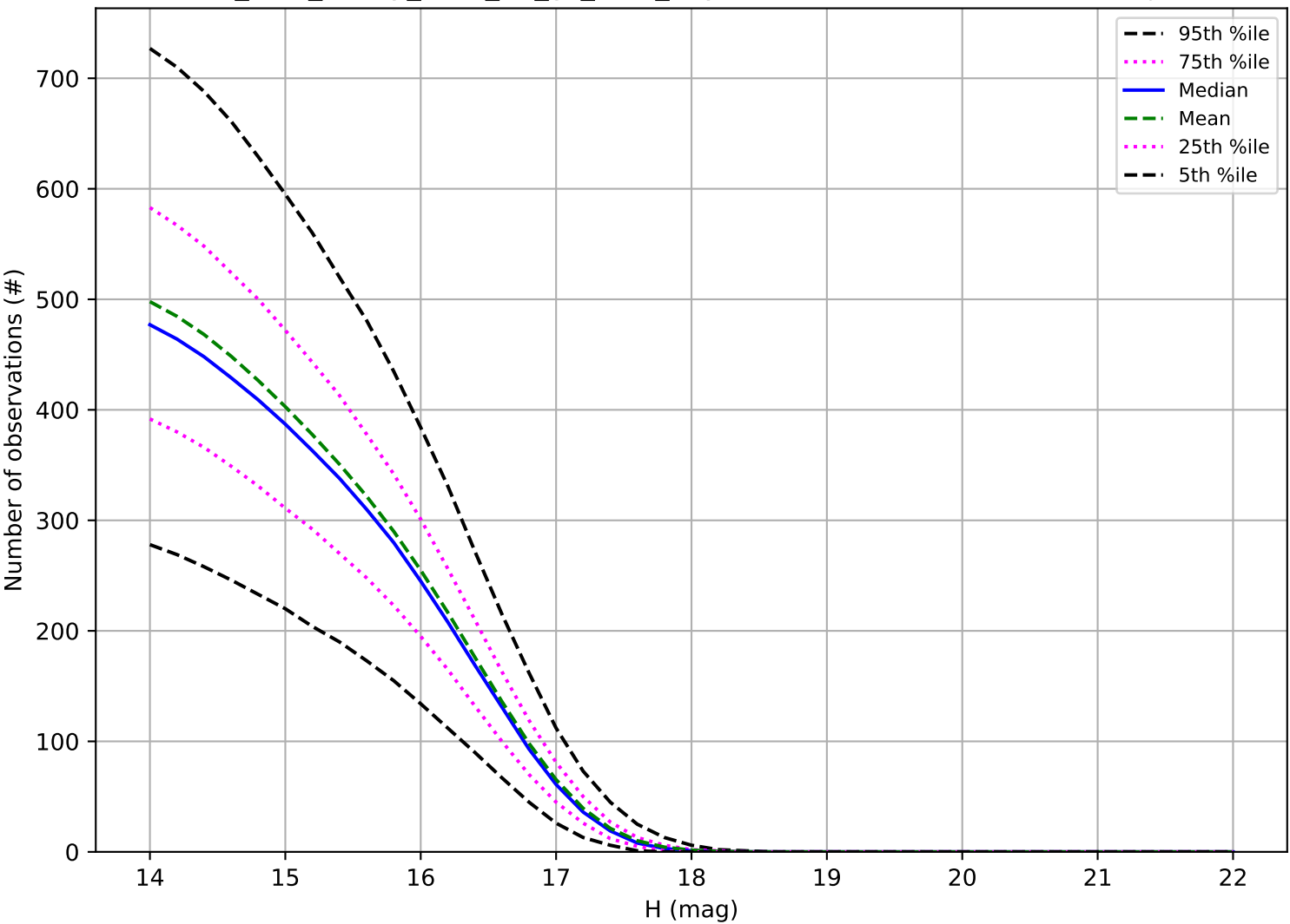
too_elab_heavy_r128_d3_gz_v3.4_10yrs: Number of observations Trojan
