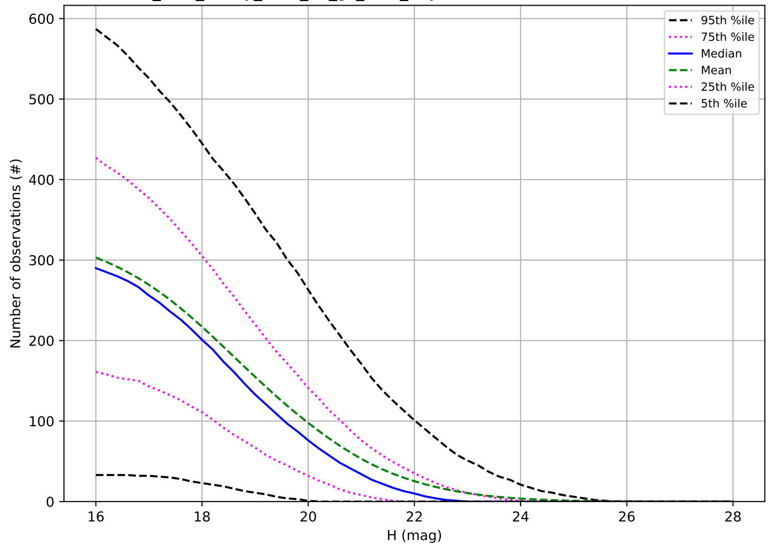
too_elab_heavy_r128_d3_gz_v3.4_10yrs: Number of observations NEO
