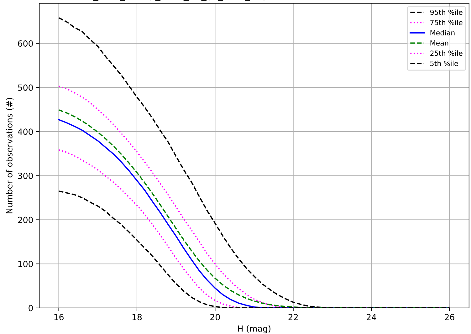
too_elab_heavy_r128_d3_gz_v3.4_10yrs: Number of observations MBA
