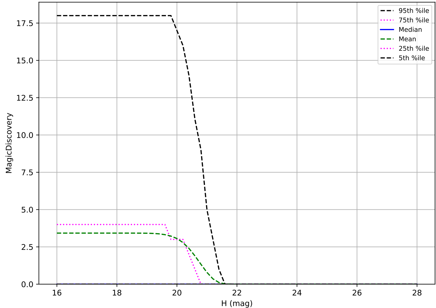
too_elab_heavy_r128_d3_gz_v3.4_10yrs: Vatira 6 detections in 60 nights detection loss
