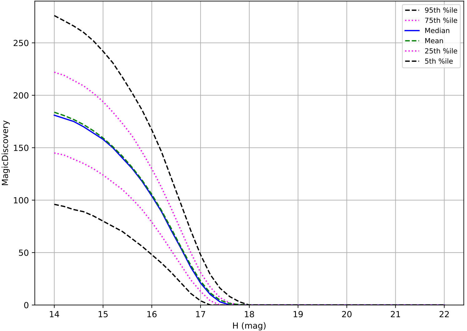
too_elab_heavy_r128_d3_gz_v3.4_10yrs: Trojan 6 detections in 60 nights detection loss
