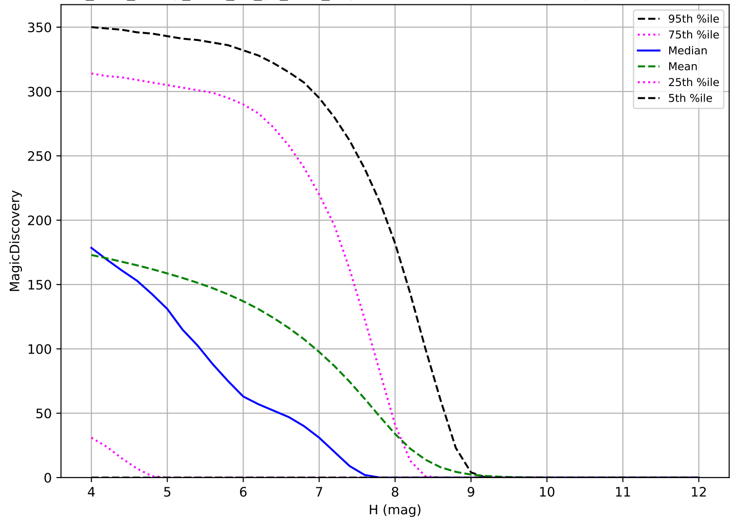
too_elab_heavy_r128_d3_gz_v3.4_10yrs: TNO 6 detections in 60 nights detection loss
