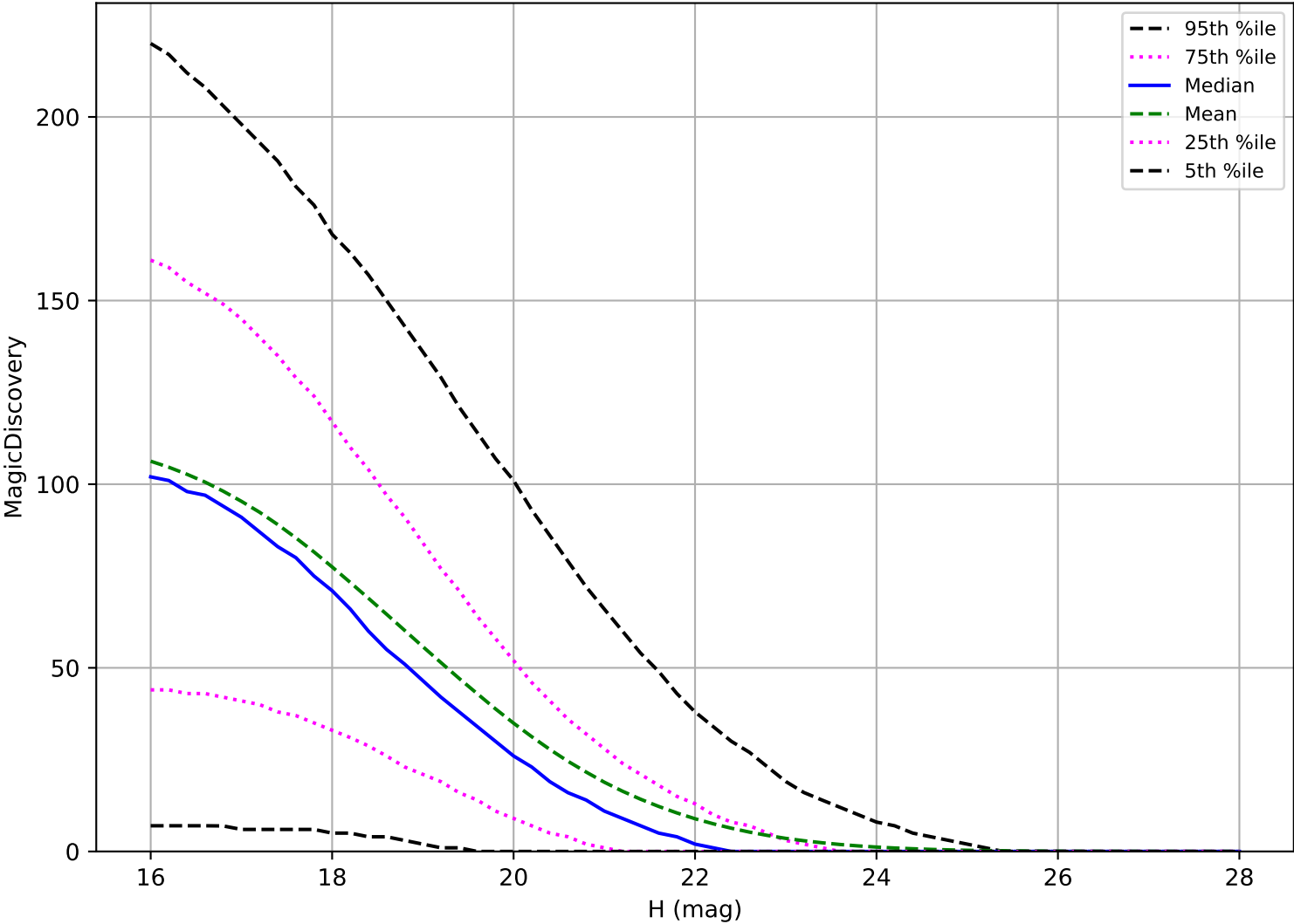
too_elab_heavy_r128_d3_gz_v3.4_10yrs: PHA 6 detections in 60 nights detection loss
