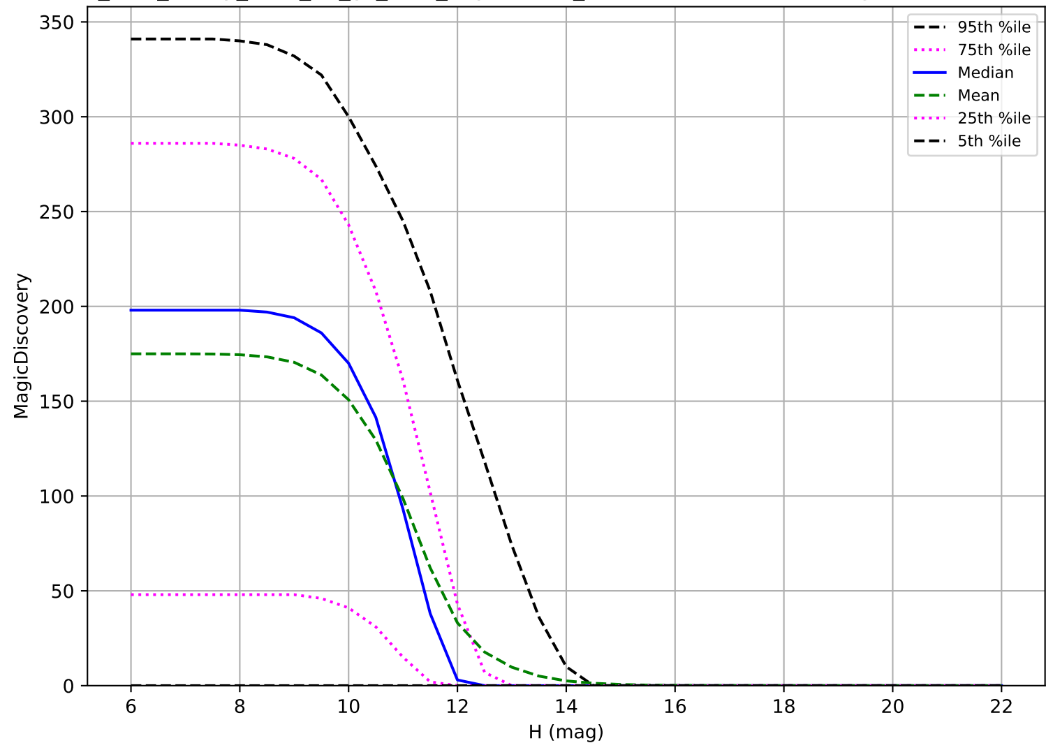
too_elab_heavy_r128_d3_gz_v3.4_10yrs: OCC_r20 6 detections in 60 nights detection loss
