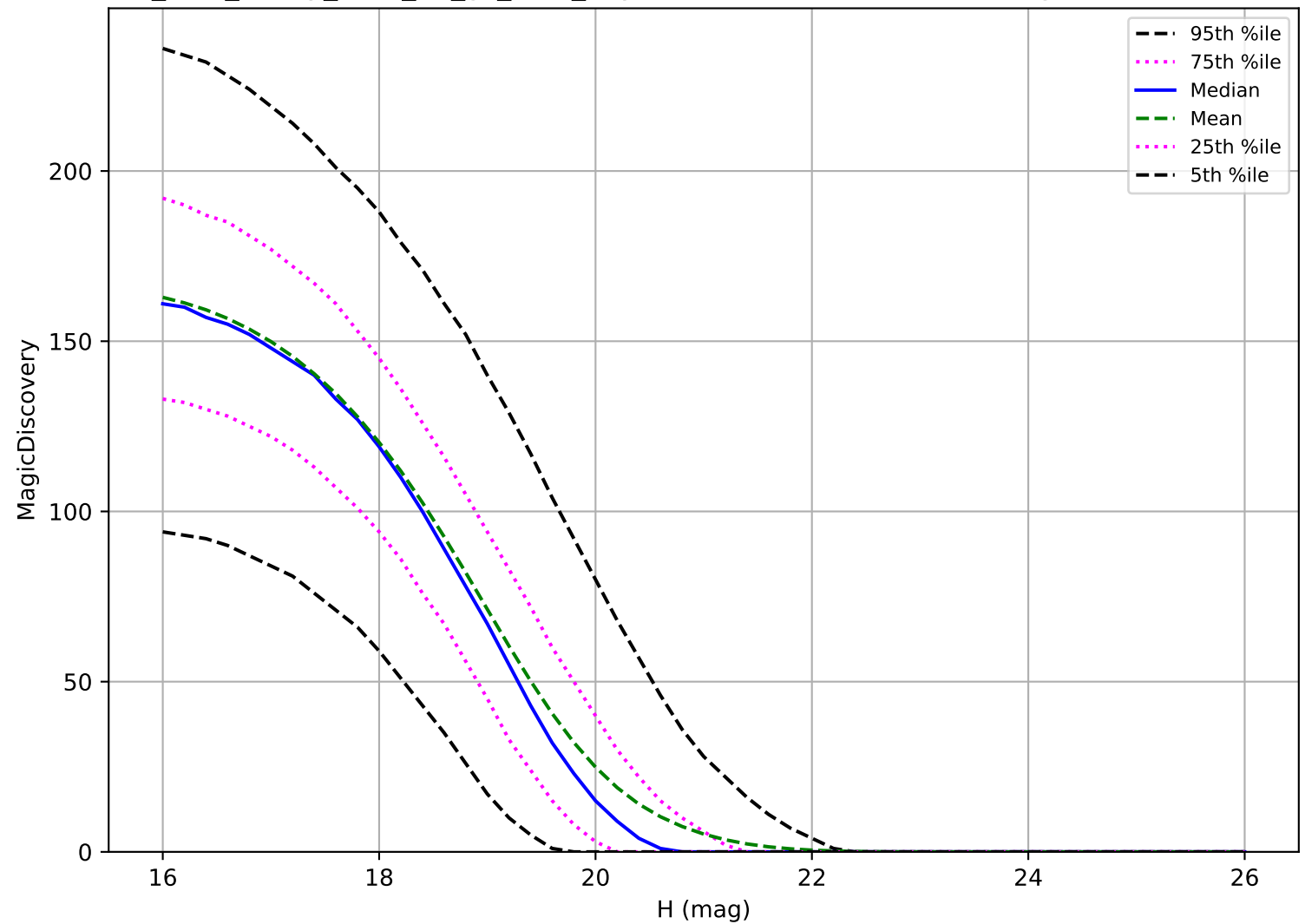
too_elab_heavy_r128_d3_gz_v3.4_10yrs: MBA 6 detections in 60 nights detection loss
