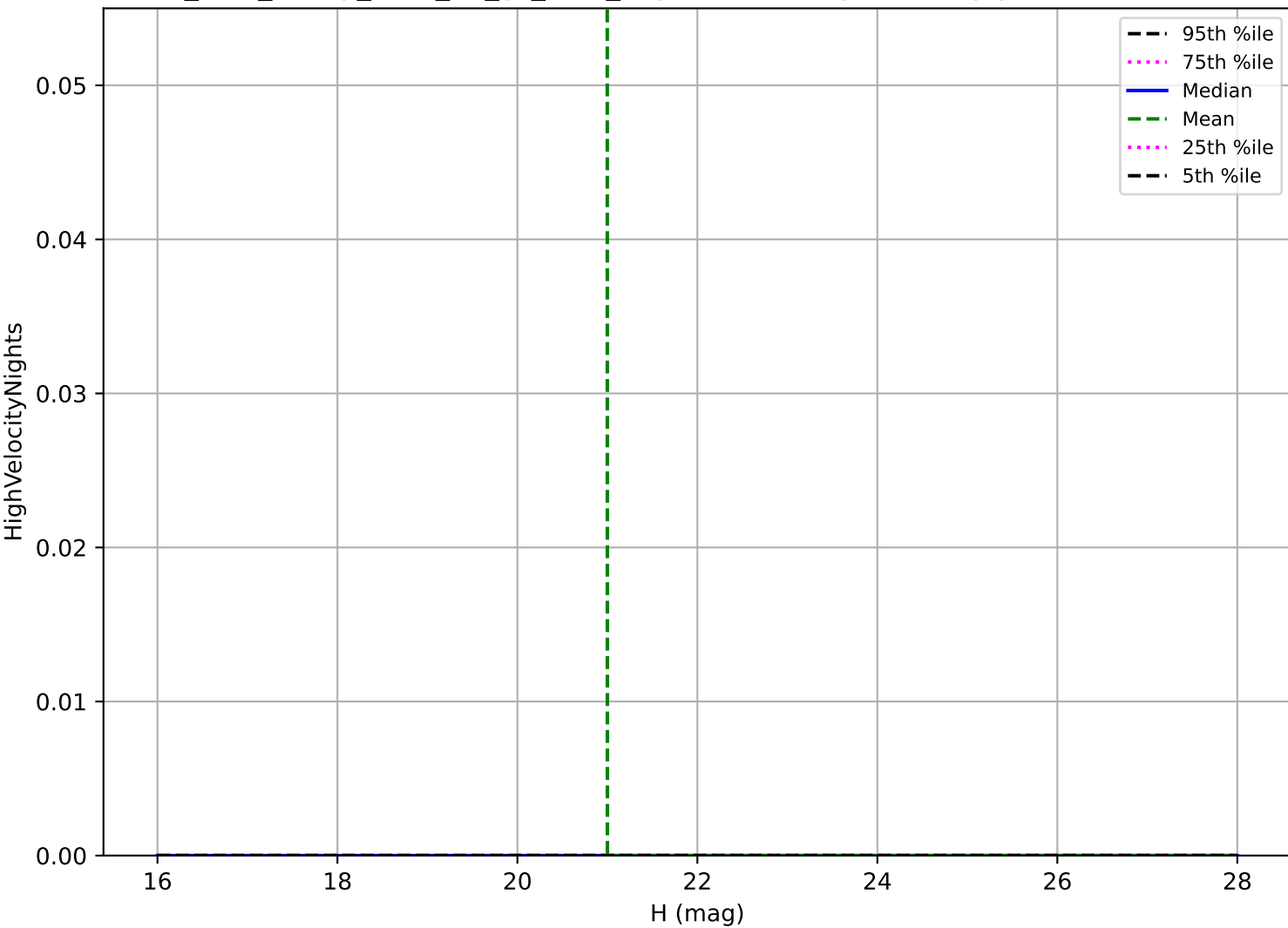
too_elab_heavy_r128_d3_gz_v3.4_10yrs: Vatira High velocity pair detection loss
