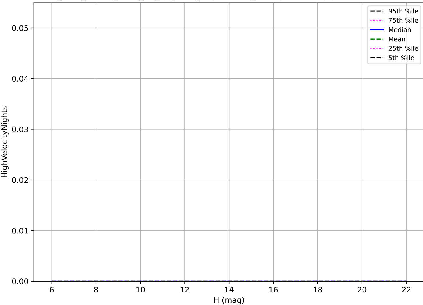
too_elab_heavy_r128_d3_gz_v3.4_10yrs: OCC_r5 High velocity pair detection loss
