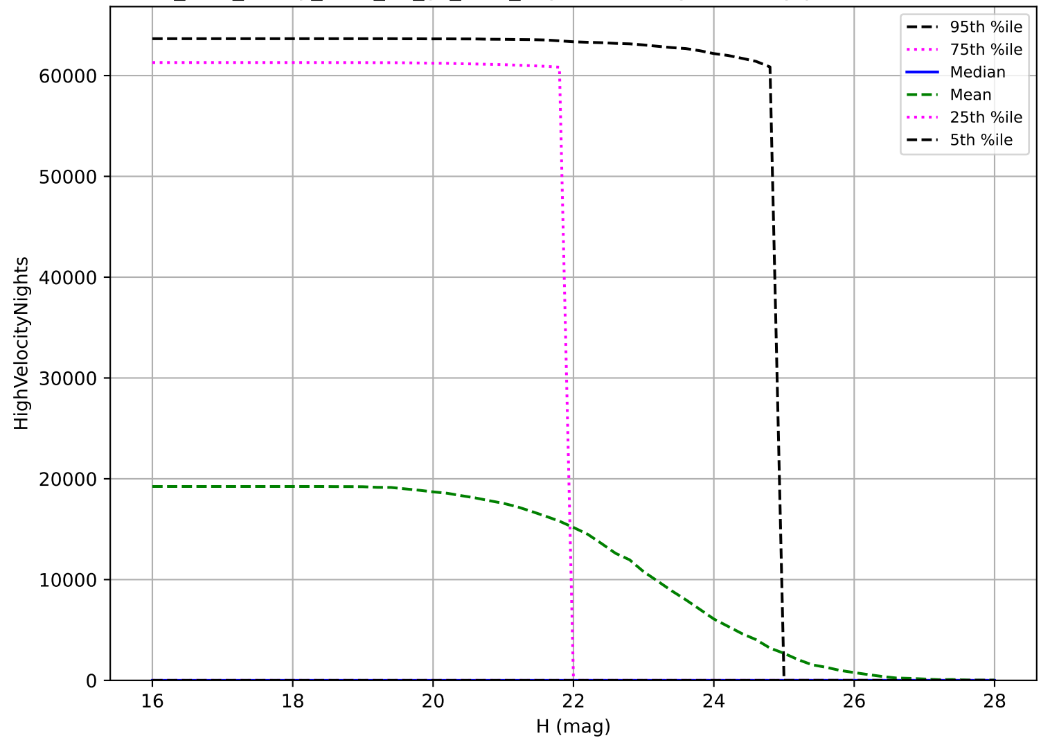
too_elab_heavy_r128_d3_gz_v3.4_10yrs: NEO High velocity pair detection loss
