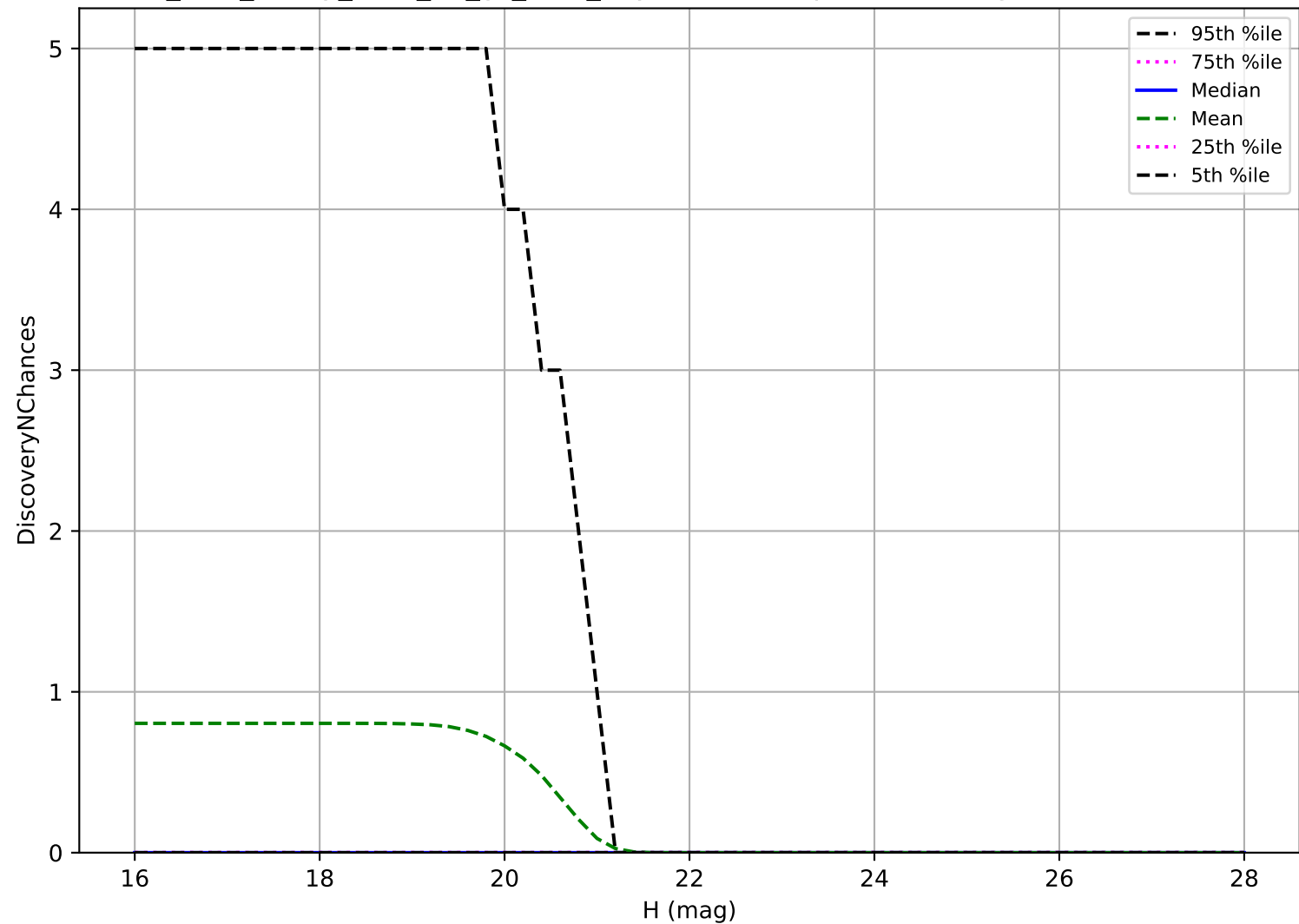
too_elab_heavy_r128_d3_gz_v3.4_10yrs: Vatira 3 pairs in 15 nights detection loss
