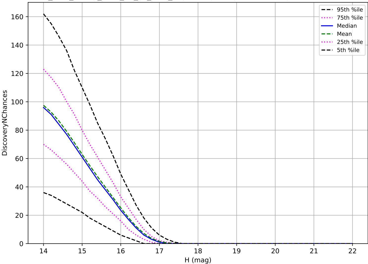
too_elab_heavy_r128_d3_gz_v3.4_10yrs: Trojan 3 pairs in 15 nights detection loss
