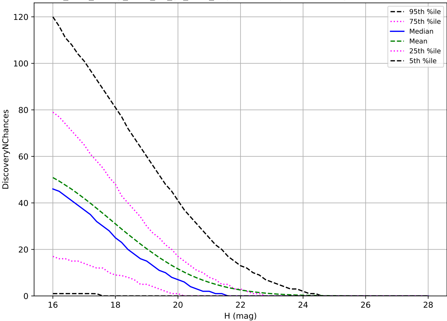
too_elab_heavy_r128_d3_gz_v3.4_10yrs: PHA 3 pairs in 15 nights detection loss
