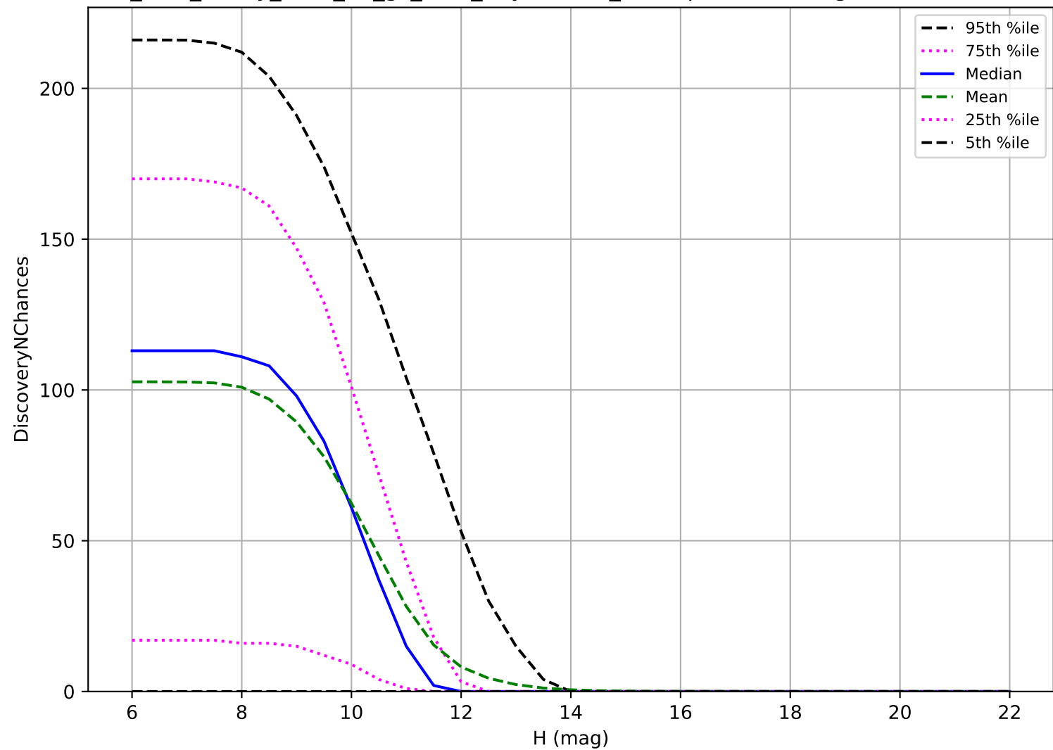
too_elab_heavy_r128_d3_gz_v3.4_10yrs: OCC_r20 3 pairs in 15 nights detection loss
