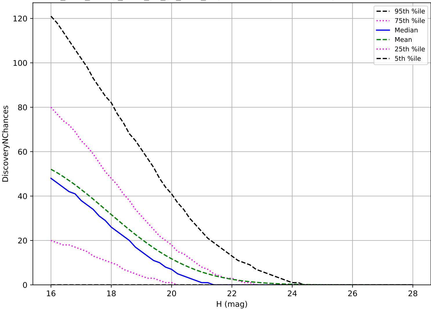
too_elab_heavy_r128_d3_gz_v3.4_10yrs: NEO 3 pairs in 15 nights detection loss
