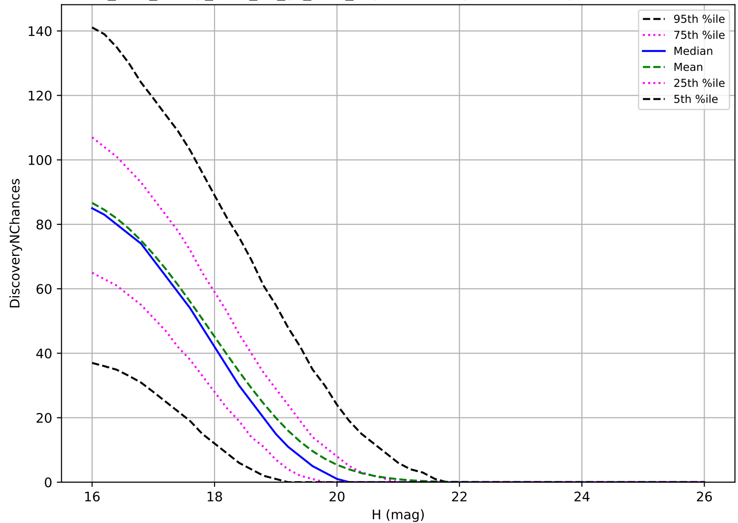
too_elab_heavy_r128_d3_gz_v3.4_10yrs: MBA 3 pairs in 15 nights detection loss
