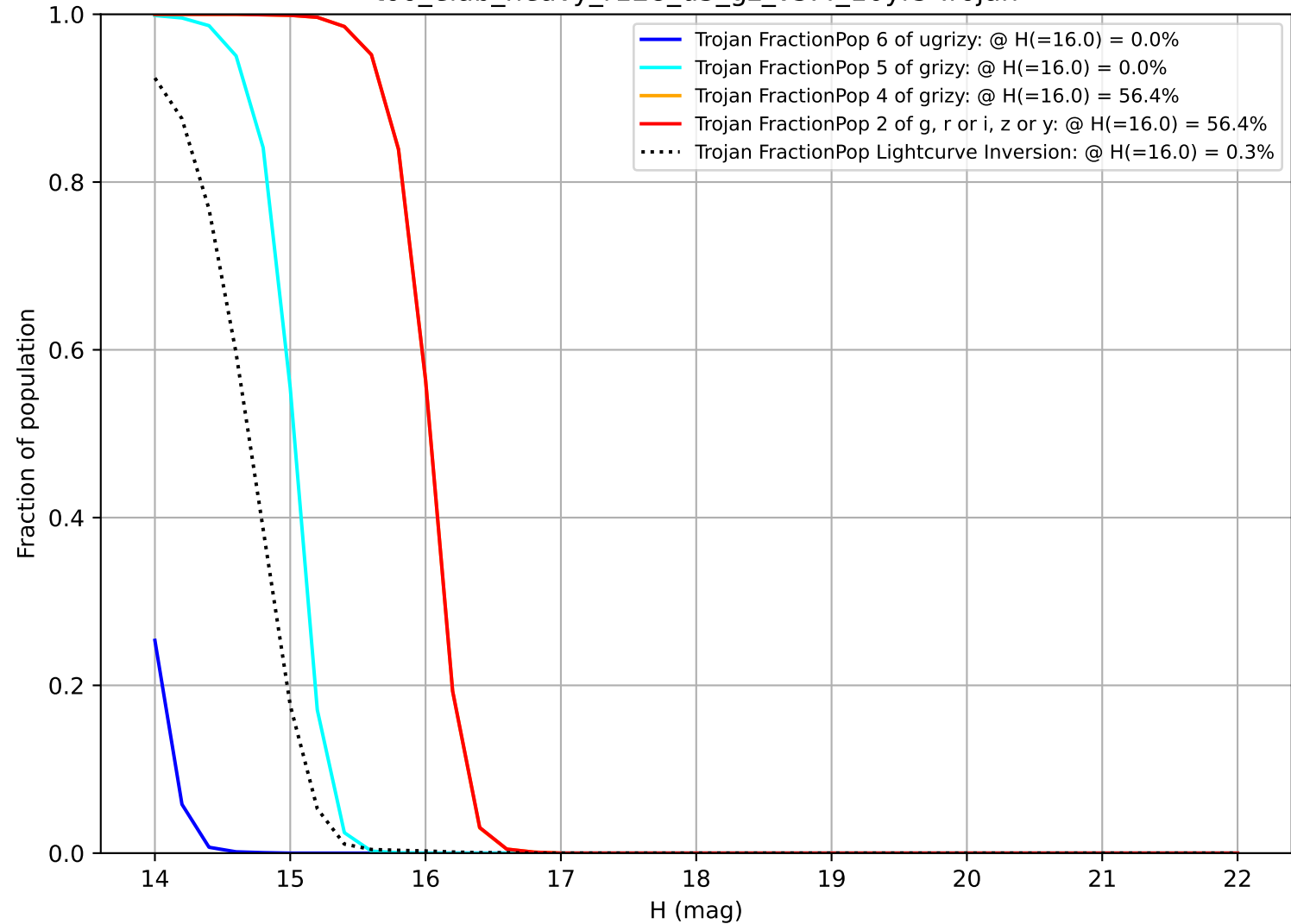
too_elab_heavy_r128_d3_gz_v3.4_10yrs Trojan
