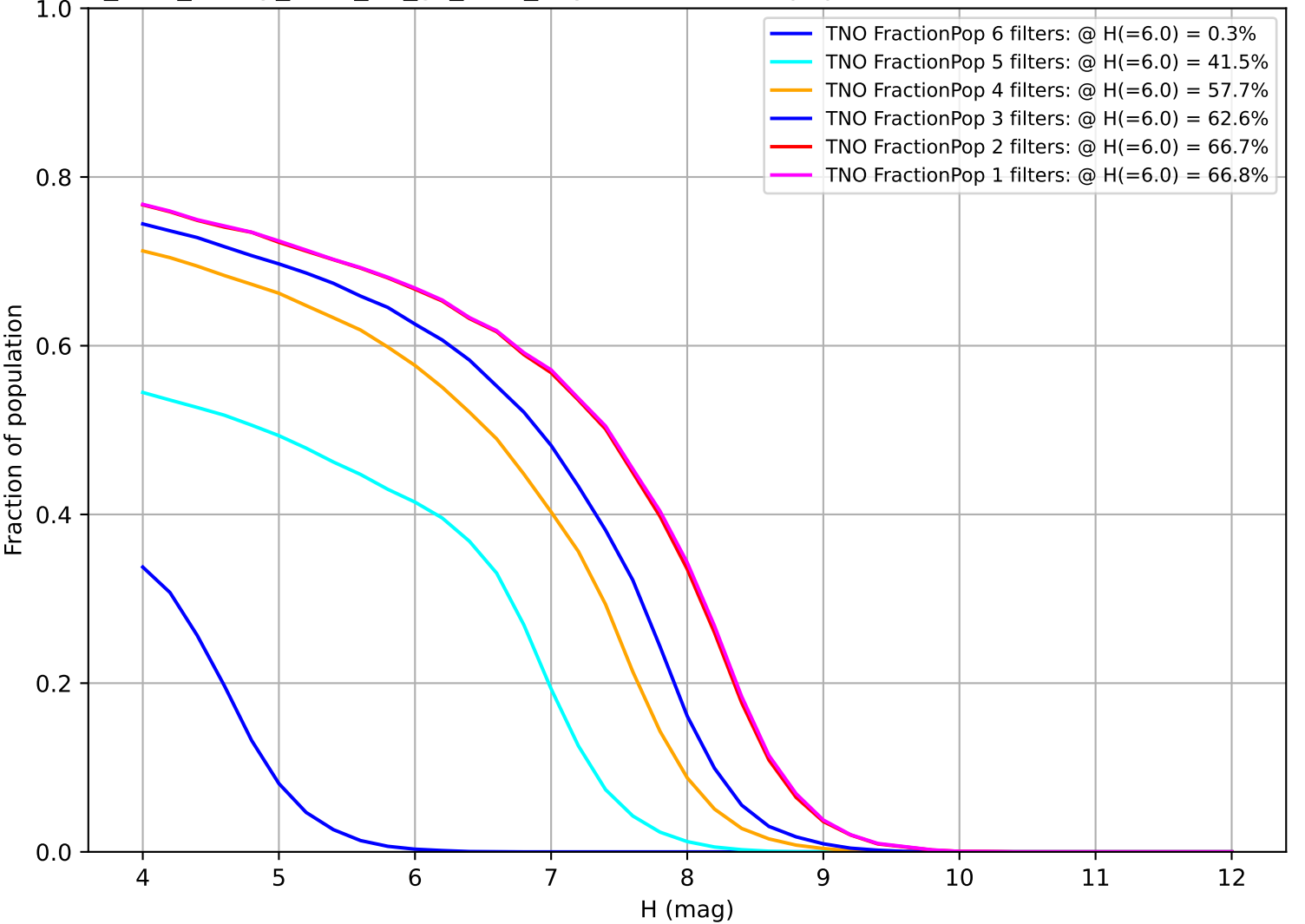
too_elab_heavy_r128_d3_gz_v3.4_10yrs: Fraction of population with colors in X filters TNO
