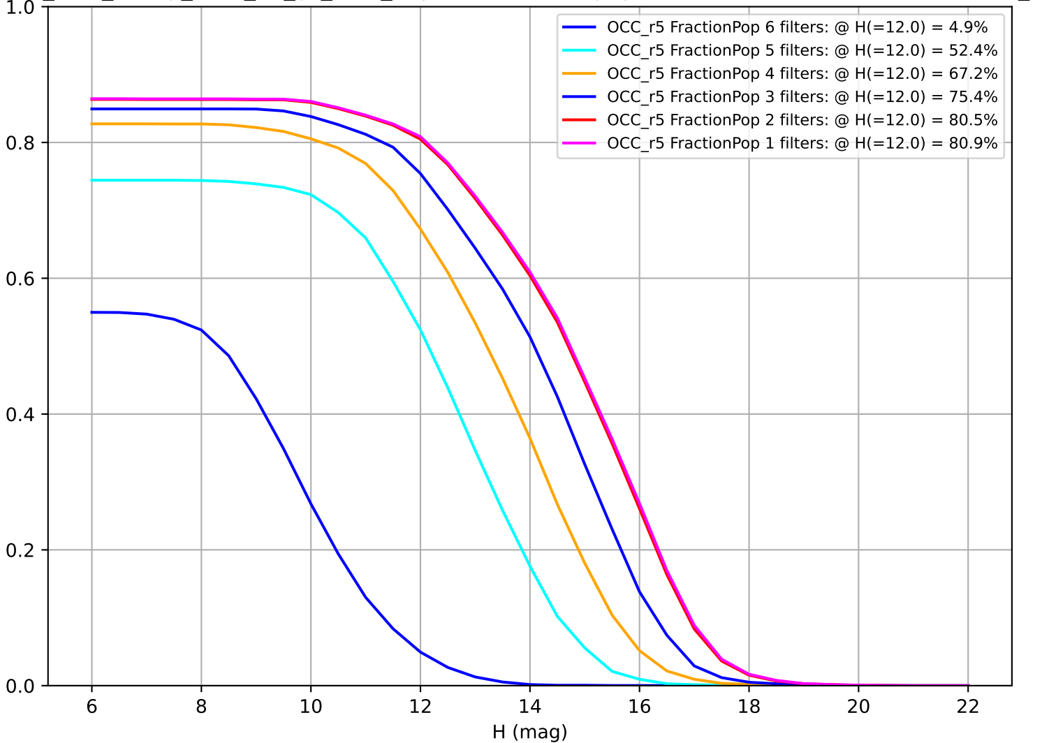
too_elab_heavy_r128_d3_gz_v3.4_10yrs: Fraction of population with colors in X filters OCC_r5
