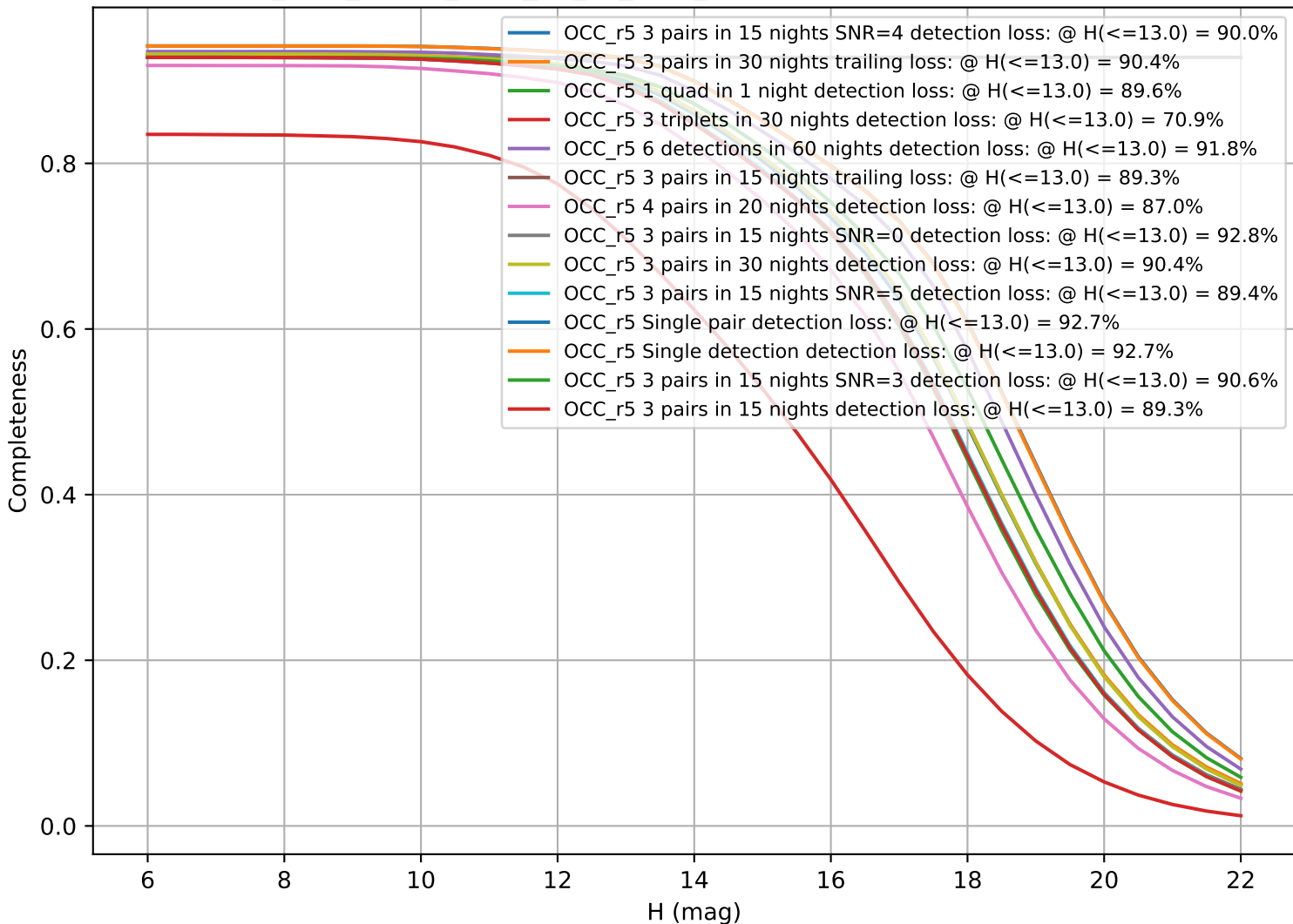
too_elab_heavy_r128_d3_gz_v3.4_10yrs: CumulativeCompleteness
