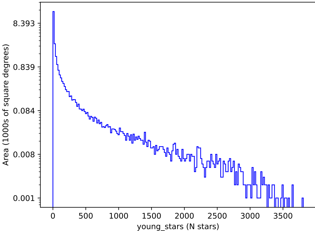
too_elab_heavy_r128_d3_gz_v3.4_10yrs : young_stars
