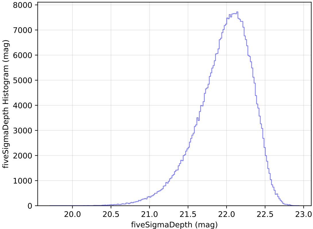
too_elab_heavy_r128_d3_gz_v3.4_10yrs y: fiveSigmaDepth Histogram
