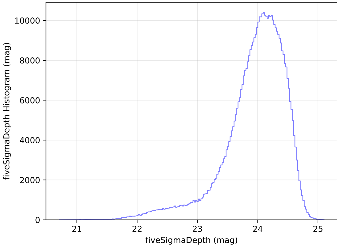
too_elab_heavy_r128_d3_gz_v3.4_10yrs r: fiveSigmaDepth Histogram
