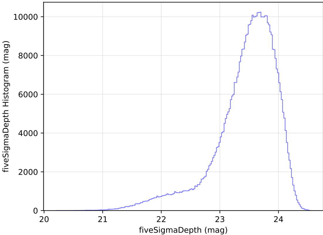
too_elab_heavy_r128_d3_gz_v3.4_10yrs i: fiveSigmaDepth Histogram
