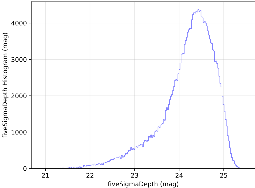
too_elab_heavy_r128_d3_gz_v3.4_10yrs g: fiveSigmaDepth Histogram
