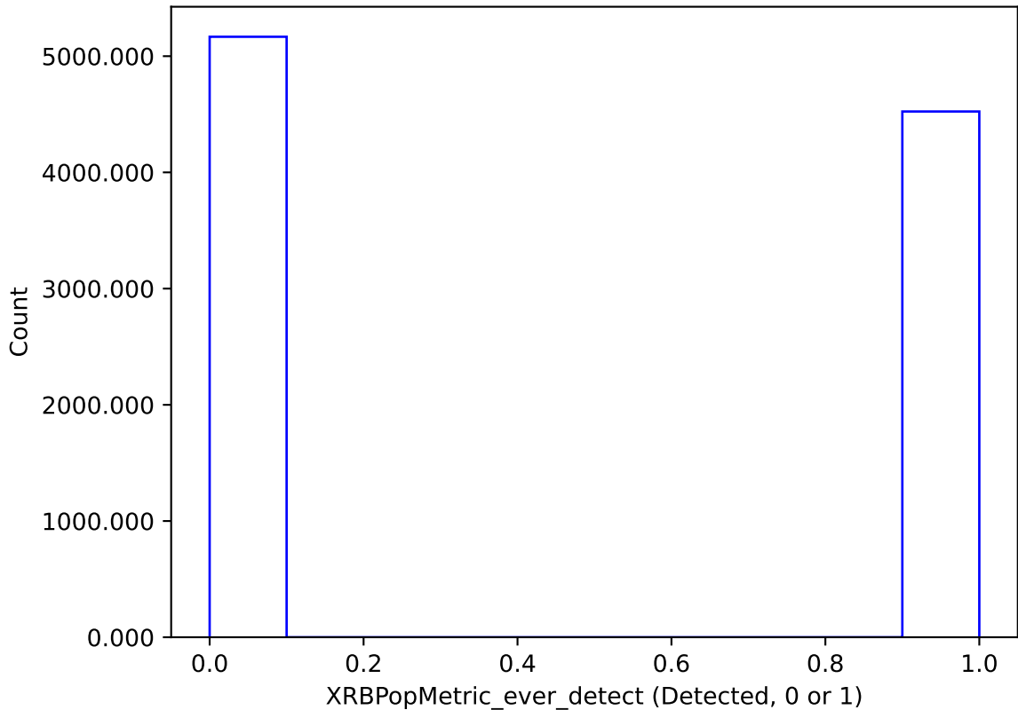
too_elab_heavy_r128_d3_gz_v3.4_10yrs : XRBPoMetric_ever_detect
