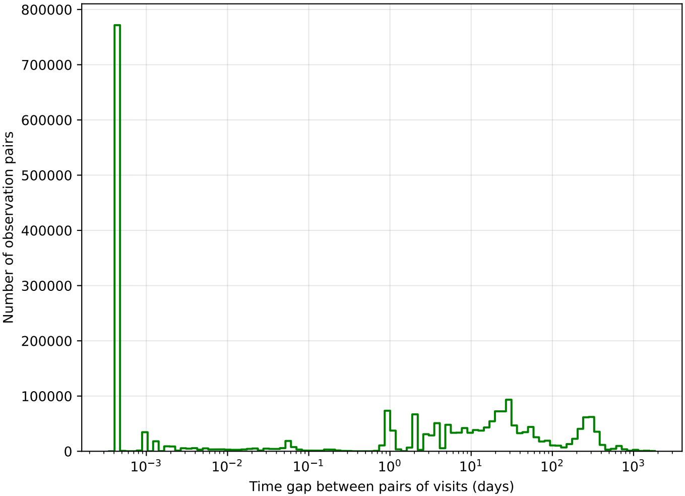
too_elab_heavy_r128_d3_gz_v3.4_10yrs g band: Tgaps observationStartMJD
