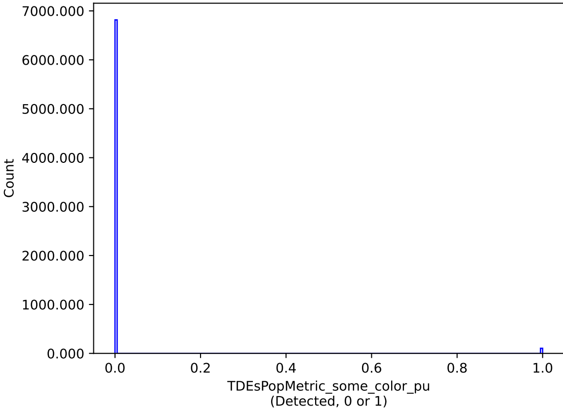
too_elab_heavy_r128_d3_gz_v3.4_10yrs : TDEsPopMetric_some_color_pu
