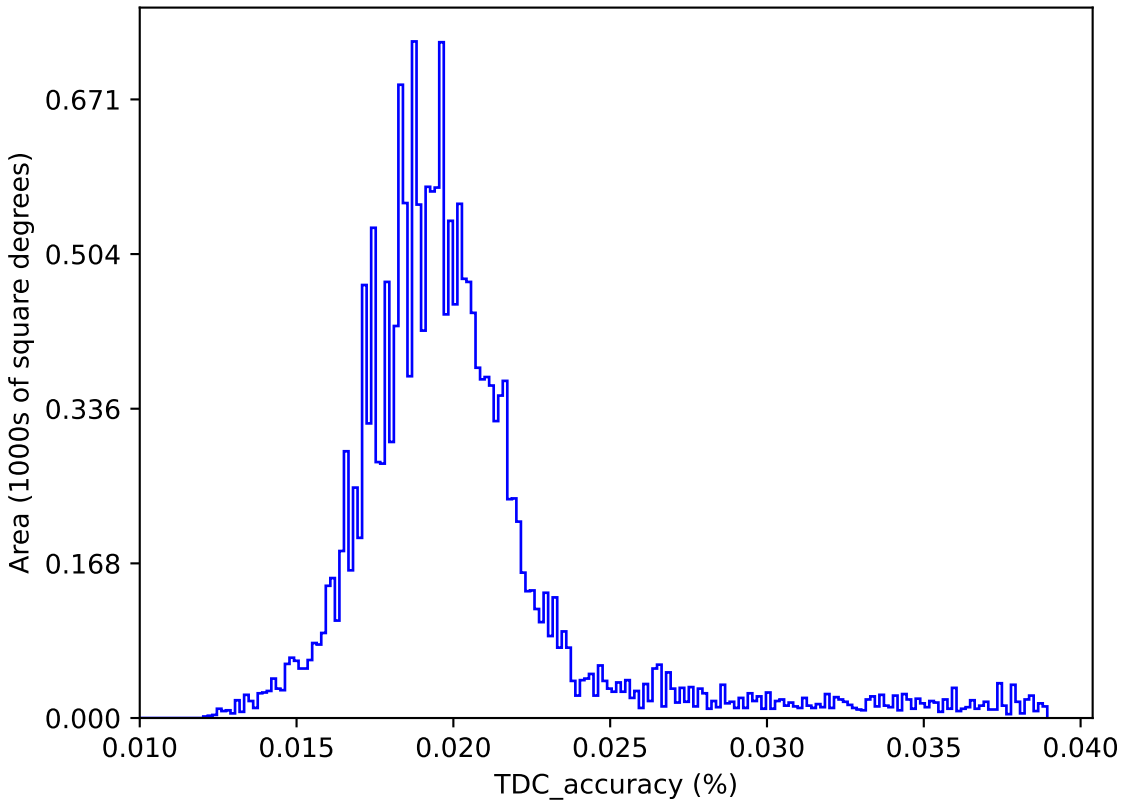
too_elab_heavy_r128_d3_gz_v3.4_10yrs : TDC_accuracy
