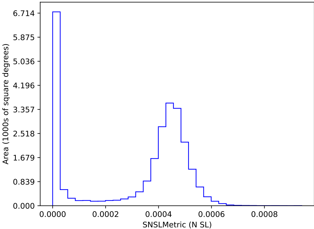
too_elab_heavy_r128_d3_gz_v3.4_10yrs : SNSLMetric
