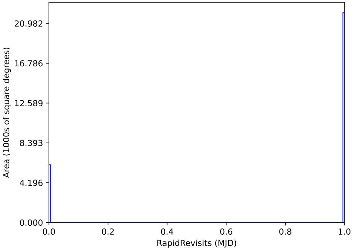
too_elab_heavy_r128_d3_gz_v3.4_10yrs : RapidRevisits
