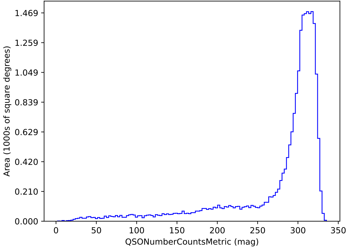
too_elab_heavy_r128_d3_gz_v3.4_10yrs u band and non-DD: QSONumberCountsMetric
